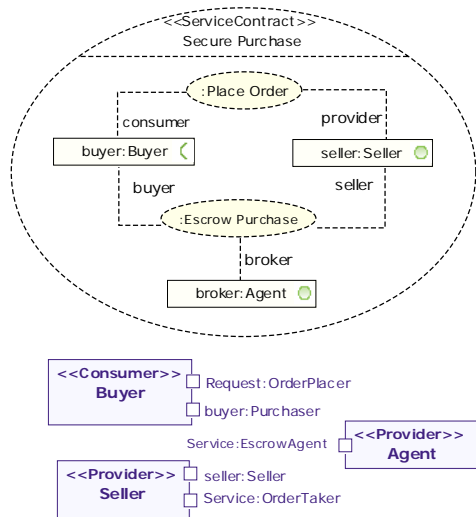
Figure 10: Specification of the Secure Purchase compound service contract which combines the two-party Place Order and the multi-party Escrow Purchase service contracts
