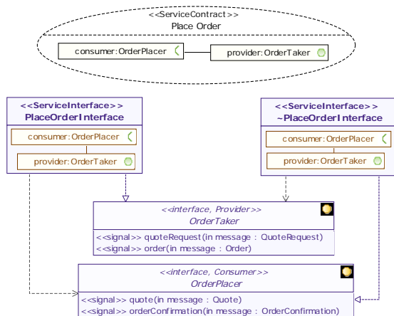
Figure 15: Service interfaces and service contracts are two different views
