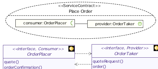
Figure 13: Service contracts models the business interfaces
