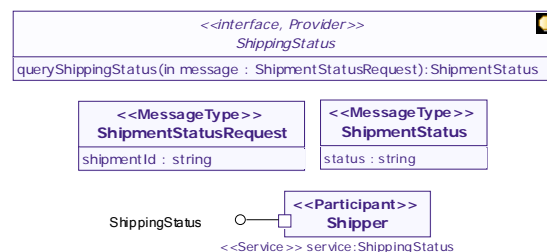
Figure 3: Specification of the Ship Status service using the simple interface based approach, consisting of a simple provider interface, its operations and message types, and the corresponding port on a participant
