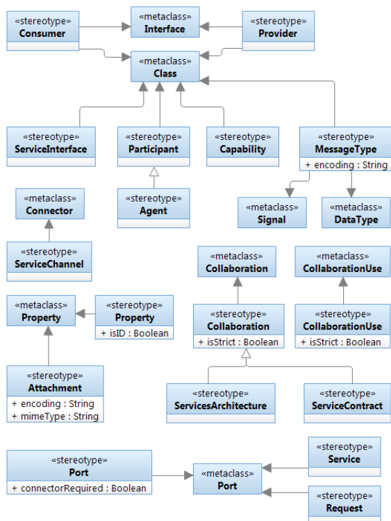
Figure 1: Main UML extensions defined as stereotypes in the UML Profile for SoaML (no relationships shown)
