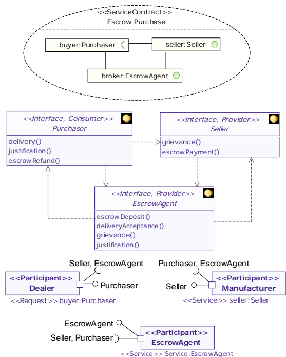
Figure 8: Specification of the Escrow Purchase service, consisting of three roles, the respective consumer interface and the two provider interface types, and the corresponding ports on the participants
