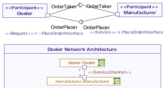
Figure 12: Consumer and provider participants connected through their request and service ports
