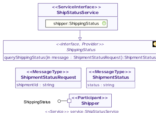
Figure 5: Specification of the Ship Status service (here named ShipStatusService ) using the service interface based approach
