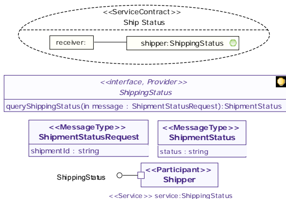
Figure 4: Specification of the Ship Status service using the service contract based approach
