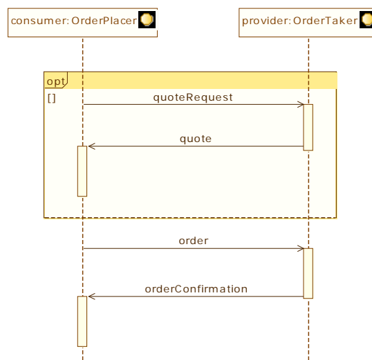
Figure 7: Specification of the Place Order service choreography (behaviour)
