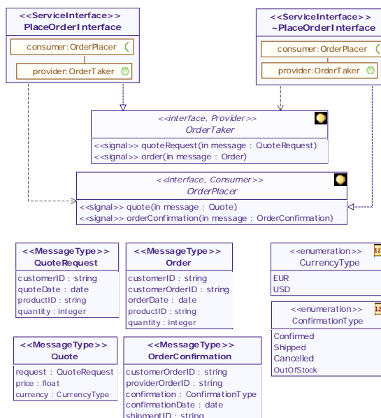
Figure 14: Service interface refines the service contract
