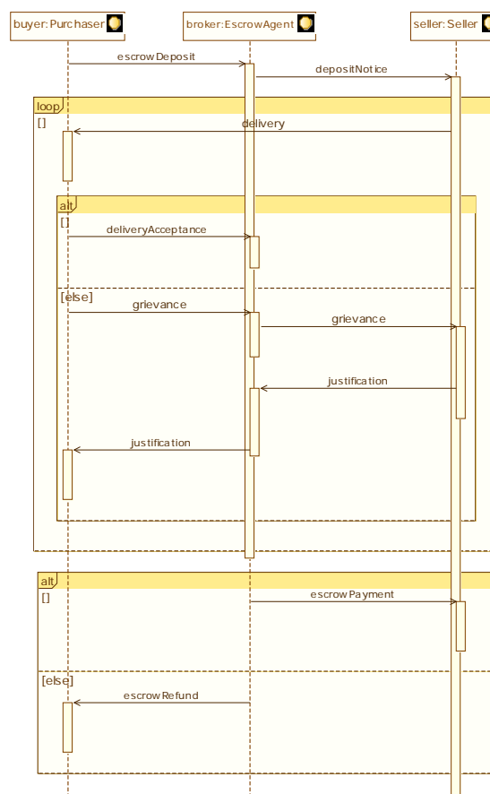
Figure 9: Specification of the Escrow Purchase service choreography (behaviour)
