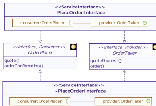
Figure 11: Specification of the Place Order service using the service interface based approach
