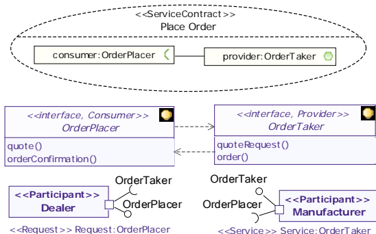
Figure 6: Specification of the Place Order service, consisting of two roles, their respective consumer and provider interface type, and the corresponding ports on the participants
