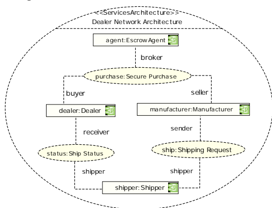
Figure 2: Services architecture for the Dealer Network Architecture illustrative example with four participants and the roles they play in the three service contract specifications
